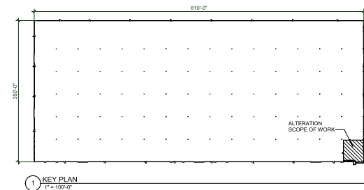
1 KEY PLAN 1" = 100'-0"
